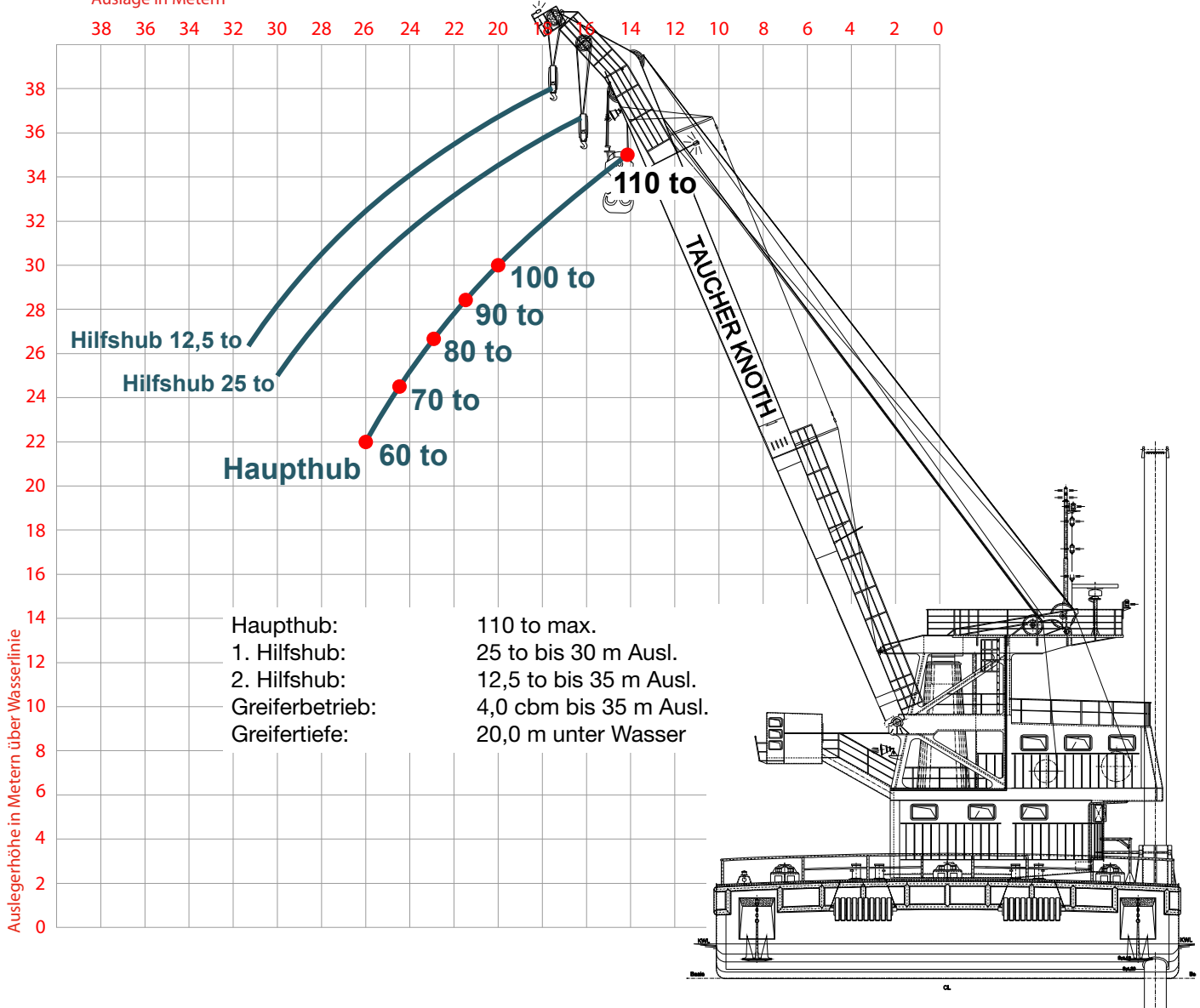
Traglastdiagramm TK-10 in to
