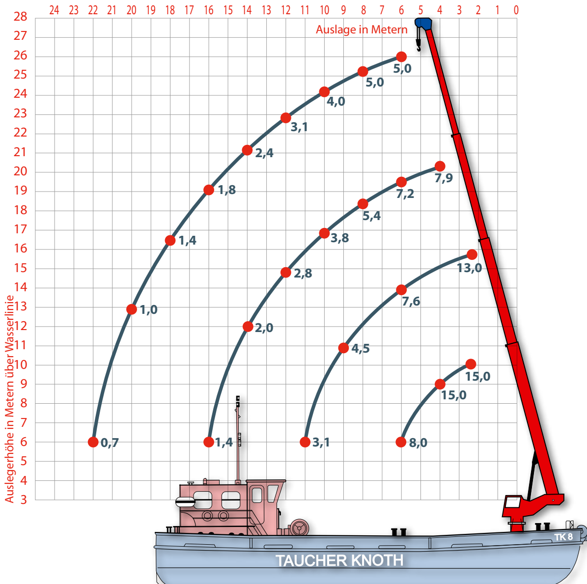
Traglastdiagramm TK-8 in to
